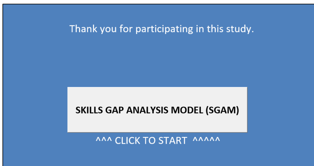
Figure 36. User Interface
