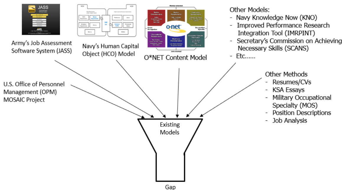
Figure 17. Literature Gap
