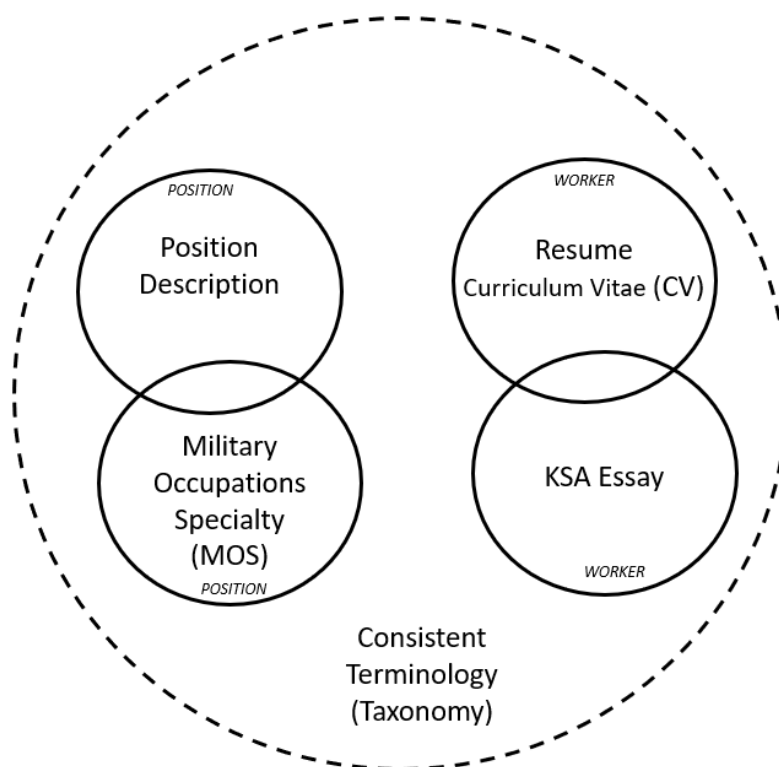
Figure 16. Terminology Issue
