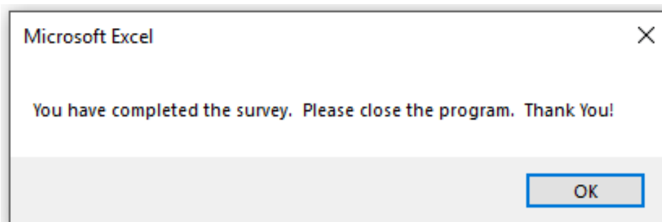
Figure 46. Survey Completion
