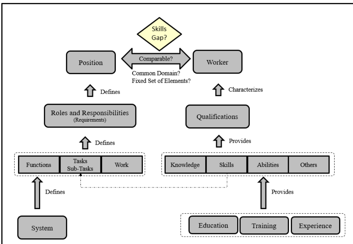
Figure 4. Domain Terminology
