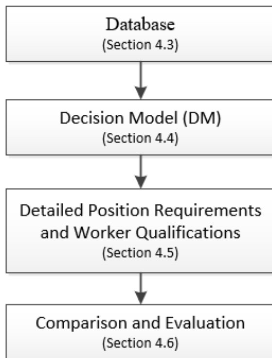
Figure 59. Adaptability Example
